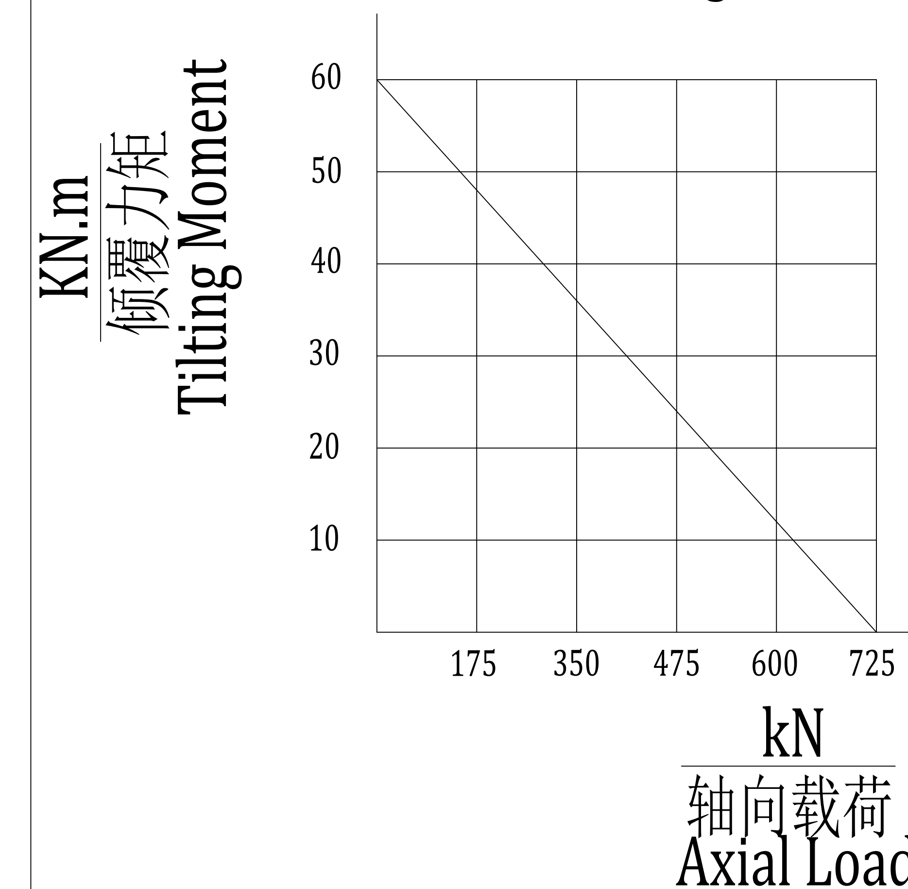
承载力矩图 MOMENT LOAD CHART 轴向载荷 & 倾覆力矩 Axial Load & Tilting Moment
