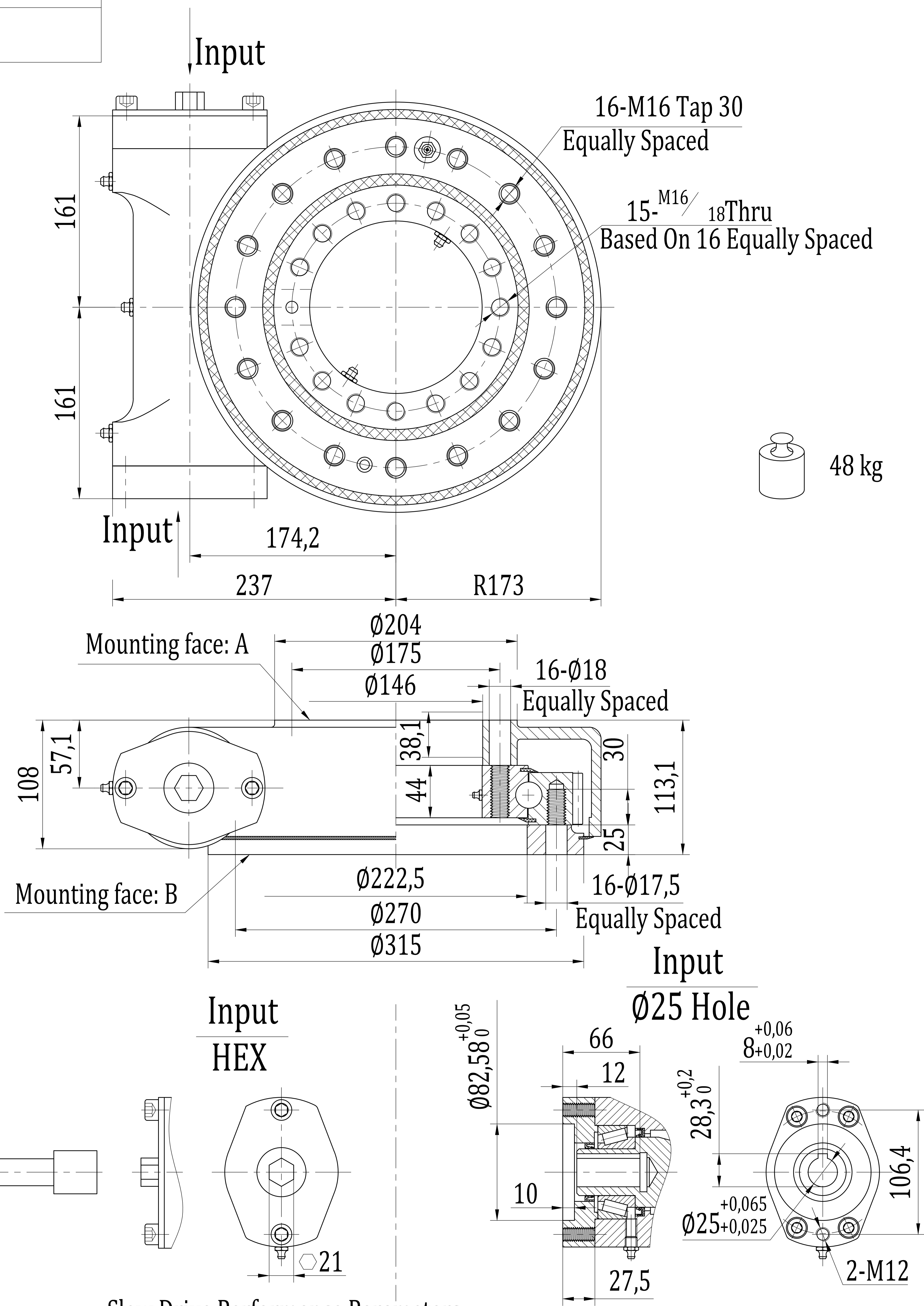
Slew Drive Performance Parameters
